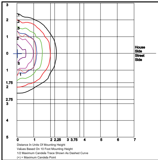
WS25GF17U5K Type IV Grid in MH MH=10 Feet
